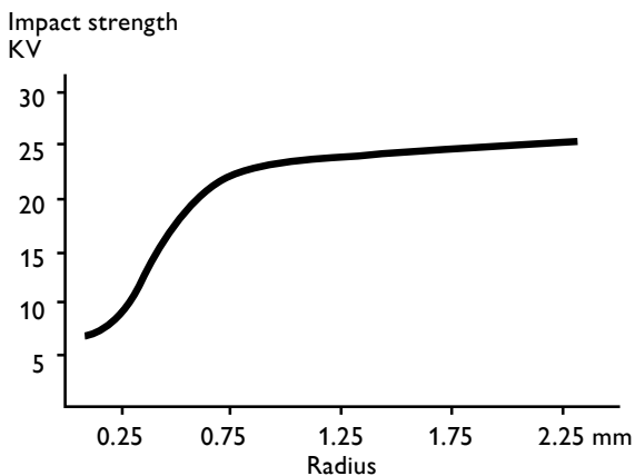
Effect of increasing radius on impact strength.
